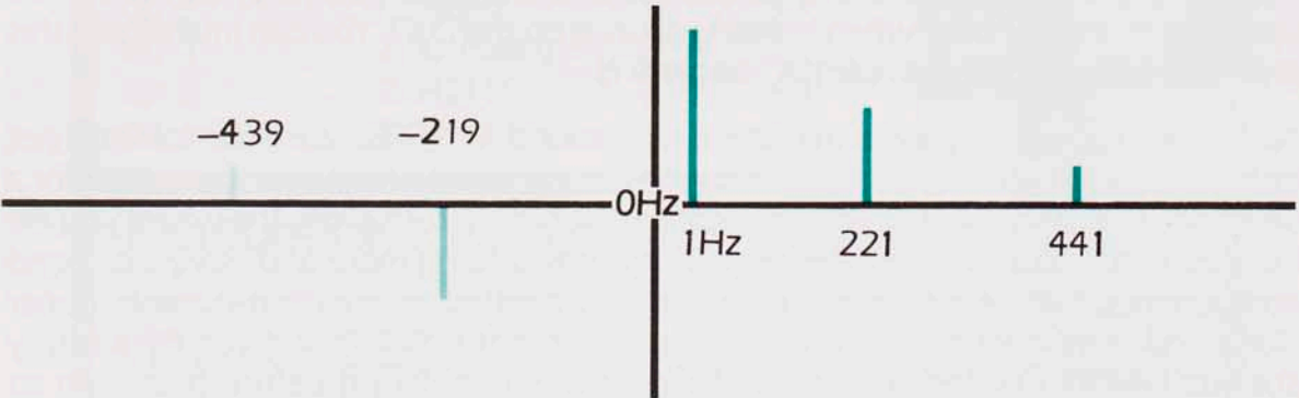
Fig. 5.7a Plot of the spectrum where f_c = 1\text{ Hz} , f_m = 220\text{ Hz} and I = 1 .
