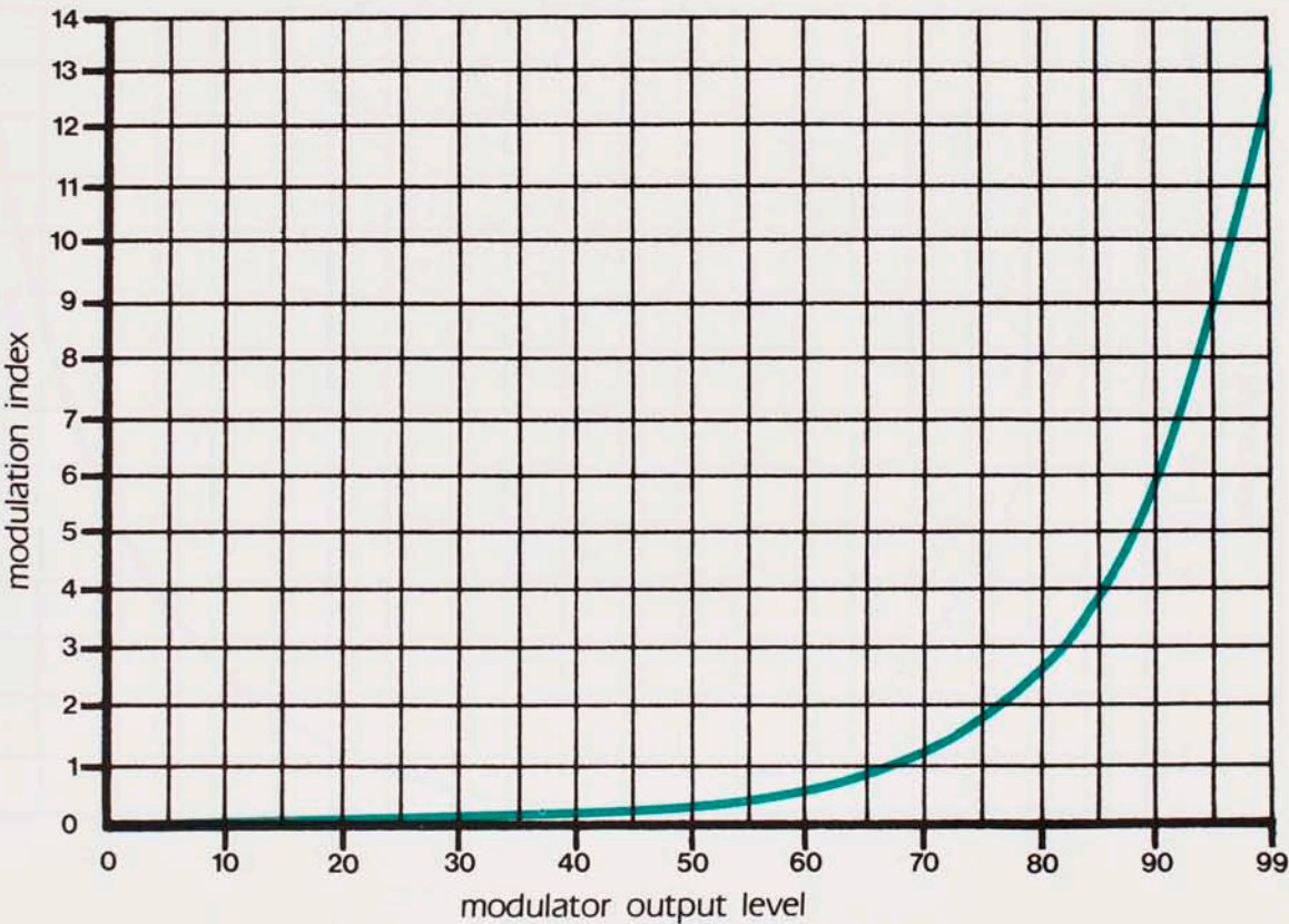
DX7——Index vs. Output Level
