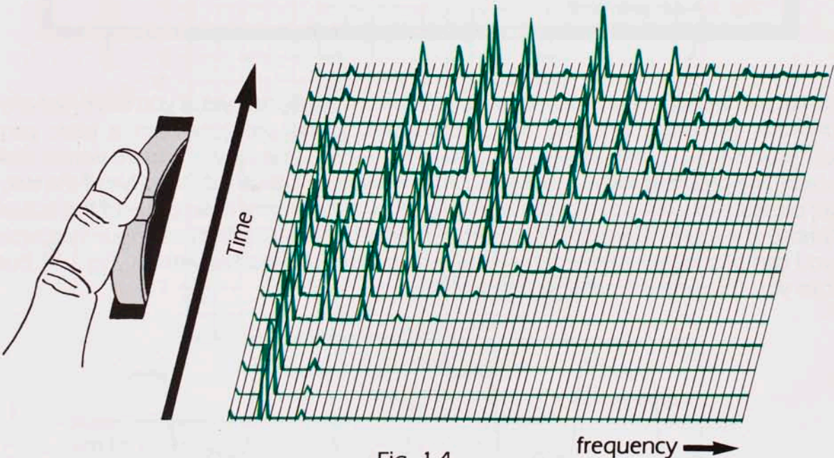
Fig. 1.4 A 3 dimensional plot showing 15 individual traces, each one showing how the sound has changed over a short period of time from the previous one. The total duration in this example is about 2 seconds, and the factor which causes the change of sound is the movement of the mod. wheel.
