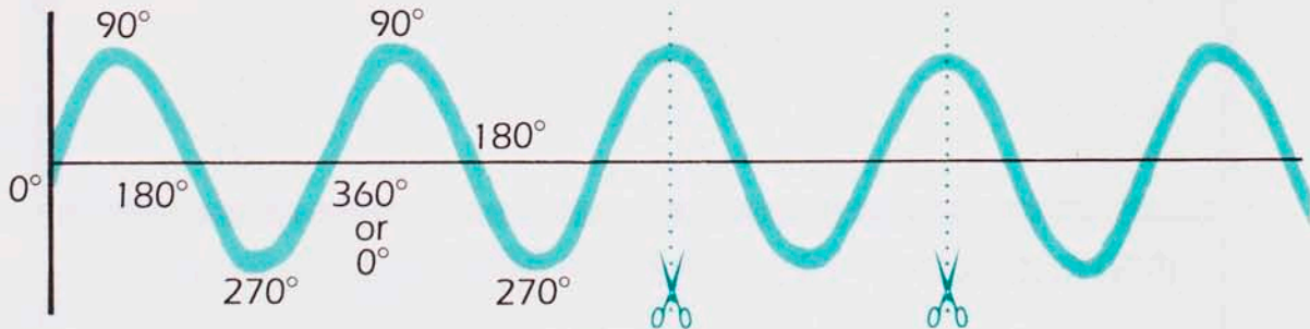
Fig. 2.9 Several periods of a sine function, where one period beginning at a phase of 90^\circ can be seen to be the same as a cosine function.
