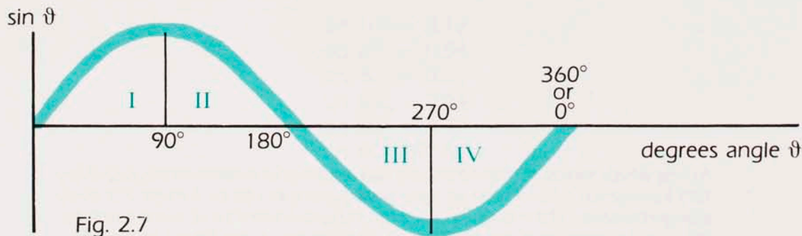
Fig. 2.7 A plot of \sin \vartheta as a function of \vartheta reveals the familiar shape of a sine wave.
