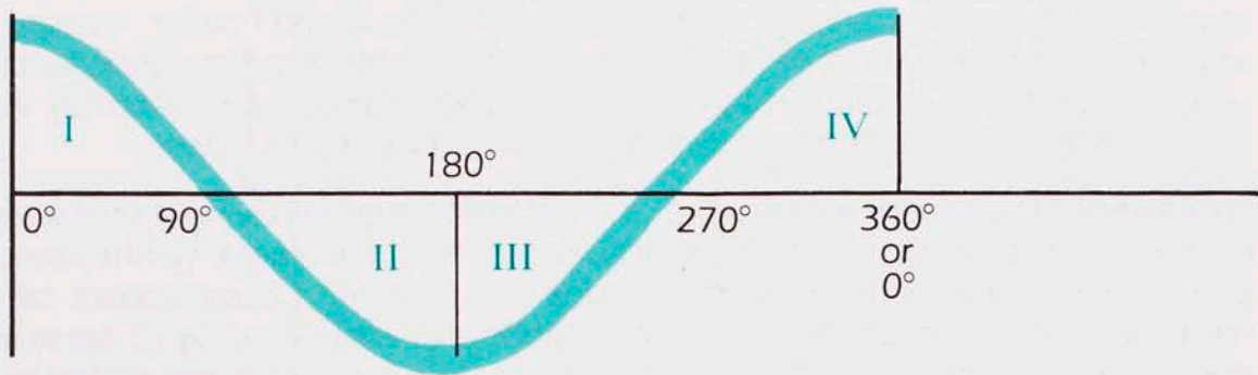
Fig. 2.8 A plot \cos \vartheta as a function of \vartheta .
